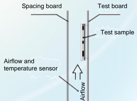
Figure 22: Wind tunnel test setup
