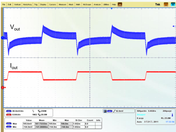
Figure 13: Output voltage dynamic response (Load: 25% - 50% - 25%, di/dt = 0.1\text{ A}/\mu\text{s} )
