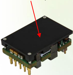
Figure 21: Thermal test point
